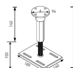
Easy connector system-R
